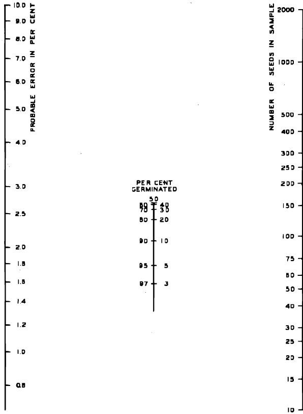
FIGURE 1. An alignment chart for finding in per cent the sampling error associated with any given sample size and percentage germination.
